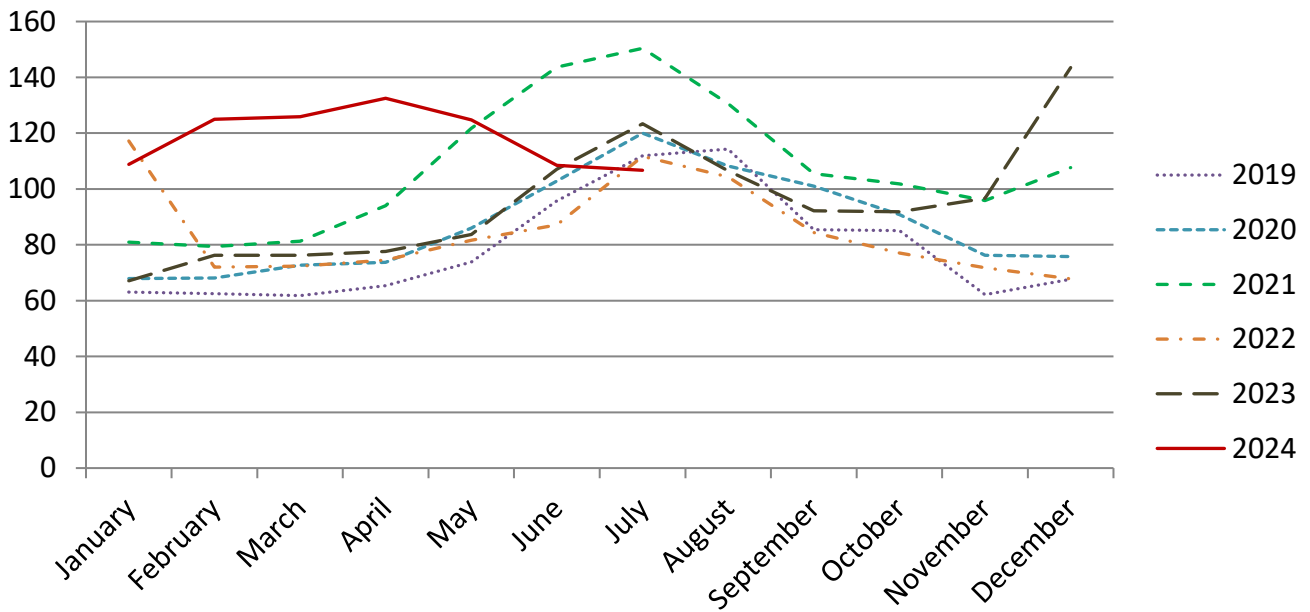
Oxenden Drinking Water System Distribution Water - Average Daily Flows
